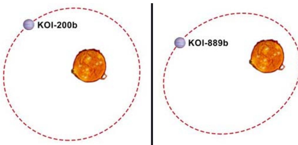
Scheme of the orbits of planets KOI-200 b (left) and KOI-988 b (right). Credit: CNRS / Ricardo Cardoso Reis (CAUP)
