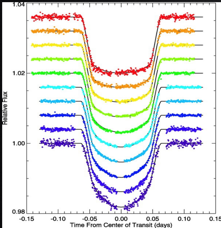
HD 209458b from 290–1030 nm (Knutson et al. 2007)
