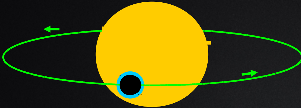
Multi-band photometry
